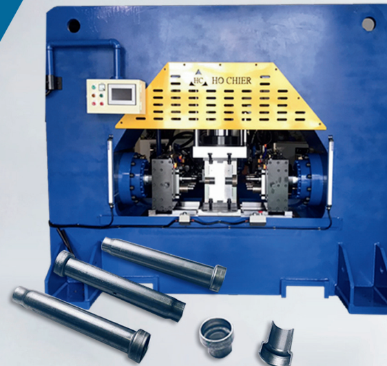
2 Ways End Forming Machine
